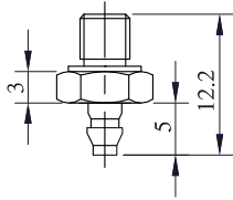
EN-PS-3B-M5 EN-PS-4B-M5
