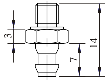
EN-PS-2~18-M5 EN-SF-8~15-M5
