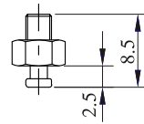
EN-PF-2/3.5-M3 EN-PJ-4-M3
