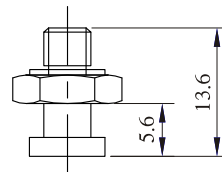
EN-PF-15-M5 EN-PJ-10~15-M5
