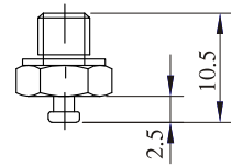
EN-PF-2/3.5-M5 EN-PJ-4-M5
