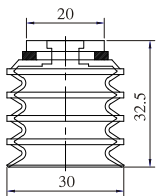
SBLE-30
