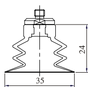
SBME-35-M5
