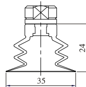
SBME-35-1/8W
