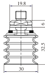
SBLE-30-1/8M
