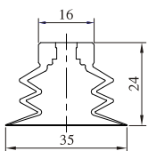
SBME-35
