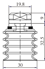
SBLE-30-1/8W
