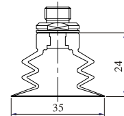
SBME-35-1/8M
