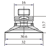
SFE-30-1/8M
